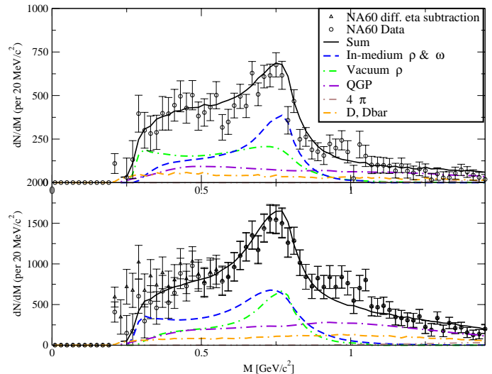
FIG. 2: Mass spectrum in semi-central In-In collisions at SPS [1] compared to theory. The lower panel shows an integration over all p_T , the upper panel one over high transverse momenta 1 \text{ GeV}/c < p_T < 2 \text{ GeV}/c . Partial contributions arise from \rho decays in vacuum after freeze-out, thermal in-medium \rho and \omega decays, radiation from a thermalized QGP and from thermal four-pion annihilation, and from correlated open charm decay.
