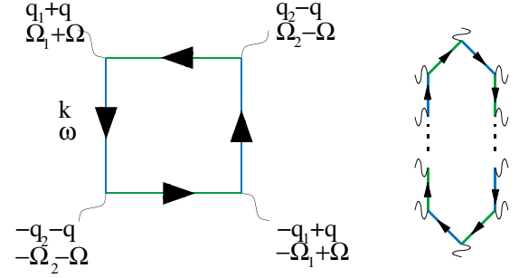
FIG. 2 (color). The diagram for the \phi^4 term in the effective bosonic action (left) and the schematic diagram for \phi^{2n} (right). Different colors show Green's functions near different hot spots.
